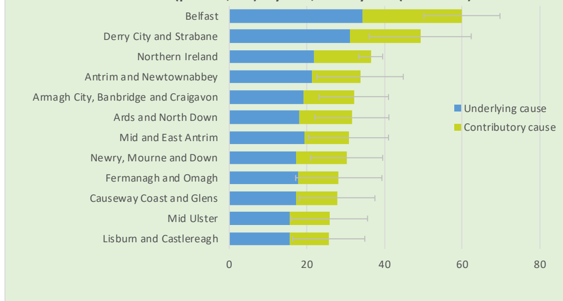
Figure 5 Alcohol-specific (Underlying and Contributory Causes) ASMRs (per 100,000) by LGD, 15-74 years (2014-2019)
