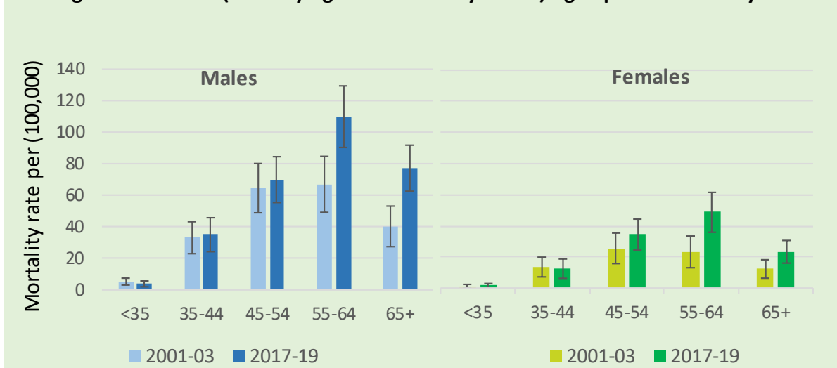
Figure 4: Alcohol (Underlying & Contributory Cause) Age-specific Mortality Rates
